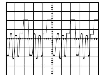
WF13 1DIV: 20V 20 sec Q503 Collector
