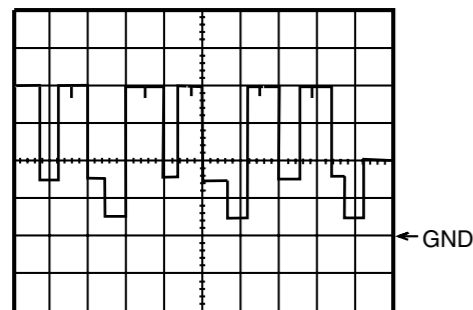
WF3 1DIV: 2V 20 sec Q501 Base
