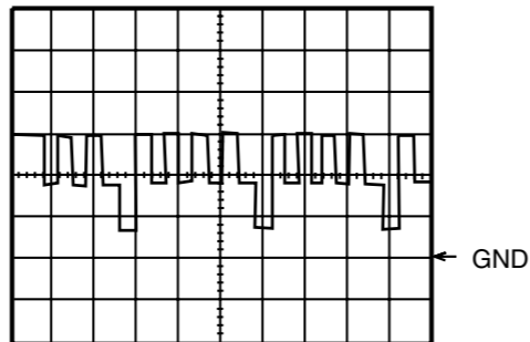
WF5 1DIV: 2V 20 sec Q 503 Base
